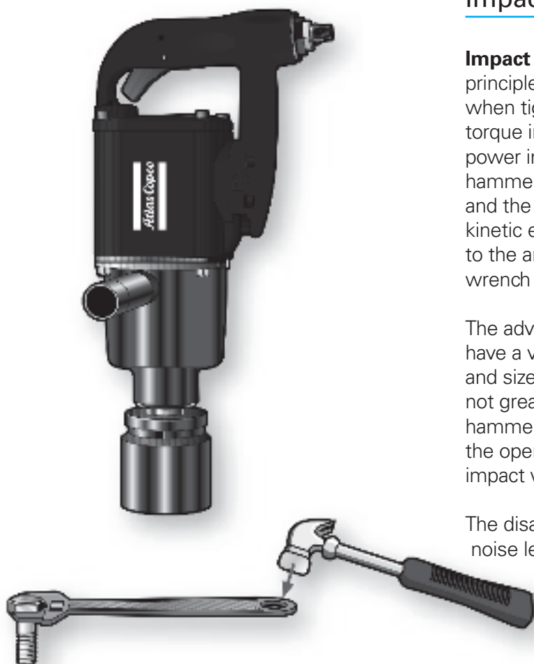
Principle of impact tools.
